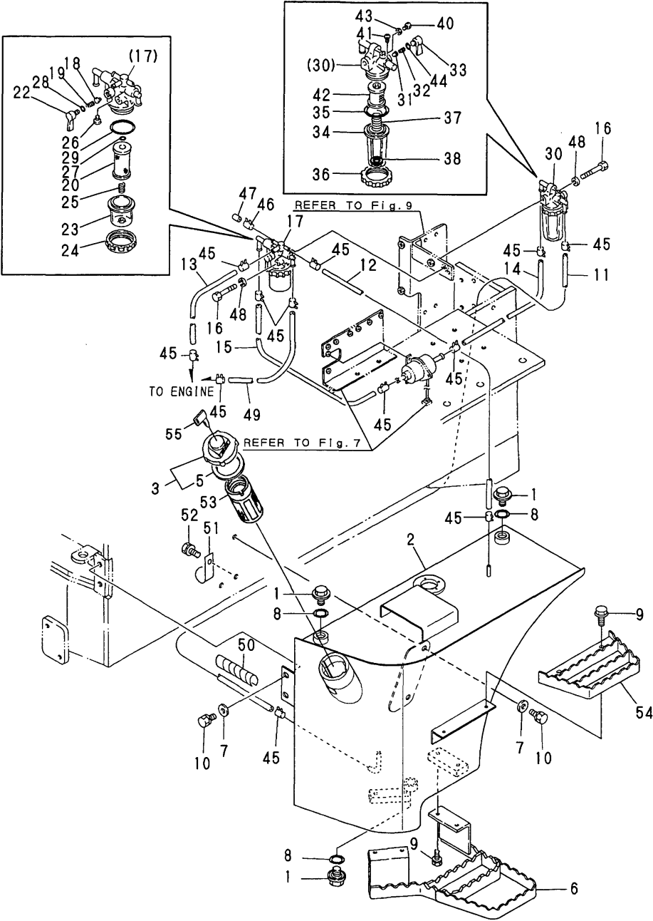
Fig.8 FUEL TANK
