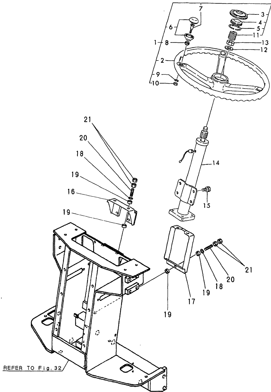
Fig.30 STEERING WHEEL & COLUMN
