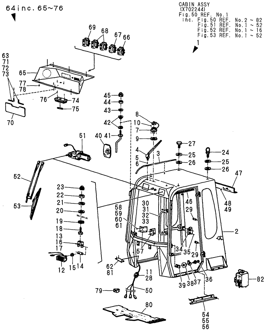
Fig.50 CABIN (1) (BODY)
