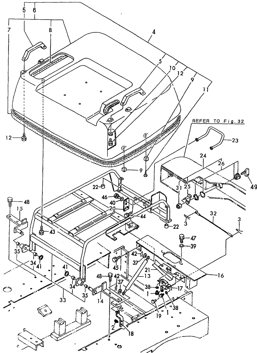
Fig.33 BONNET
