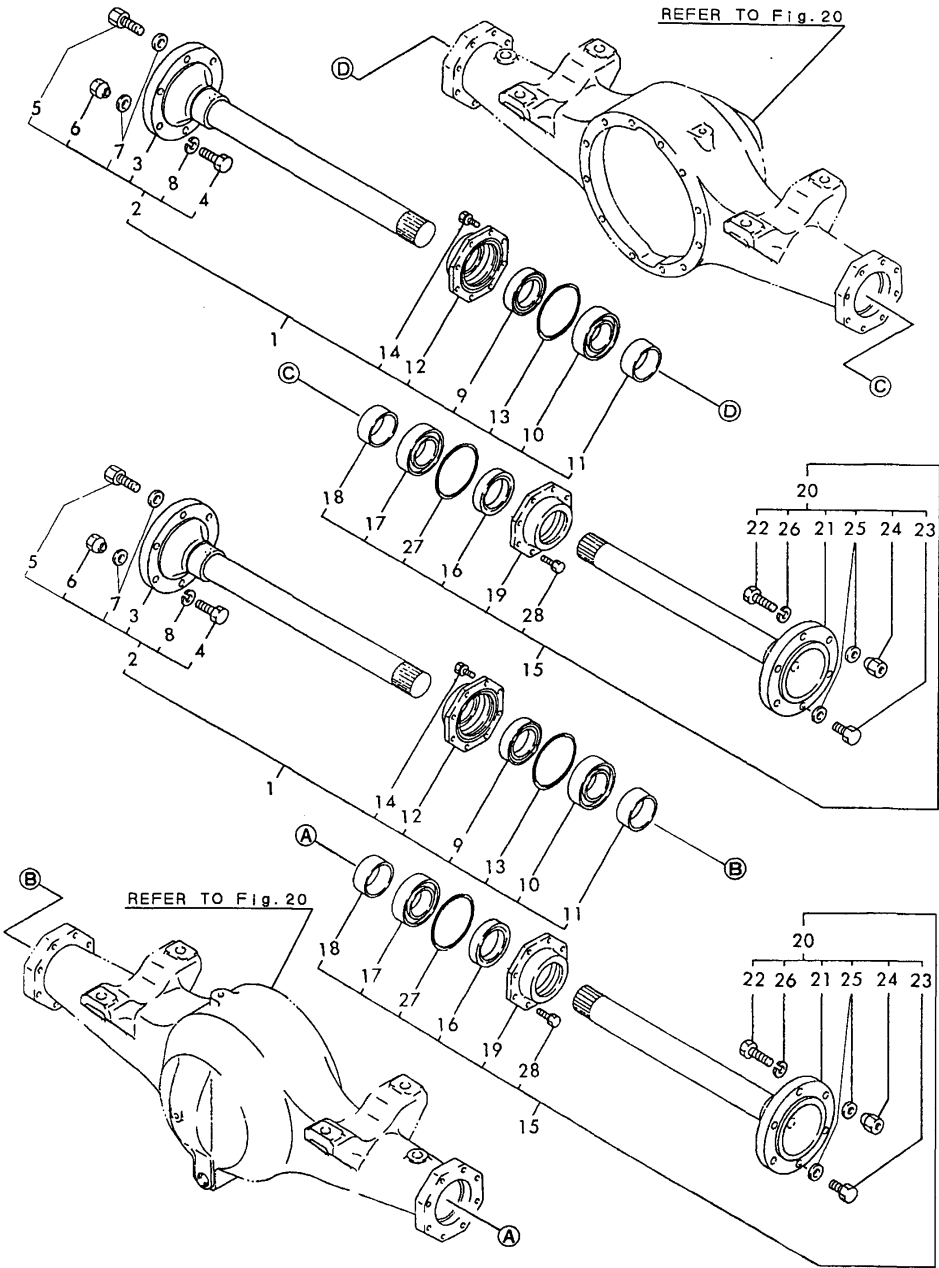
Fig. 19 AXLE SHAFT (V4-3)
