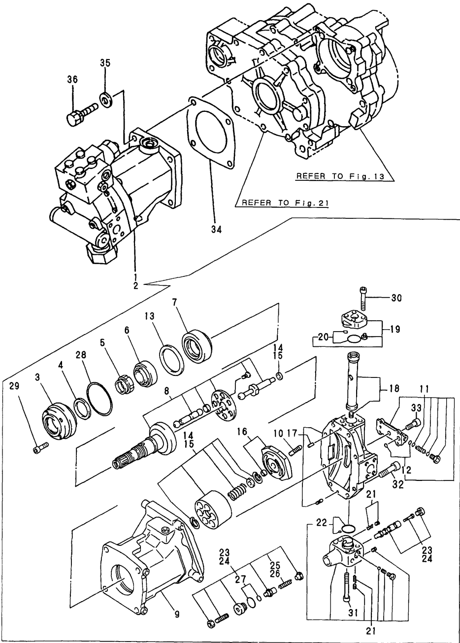
Fig.40 HST MOTOR
