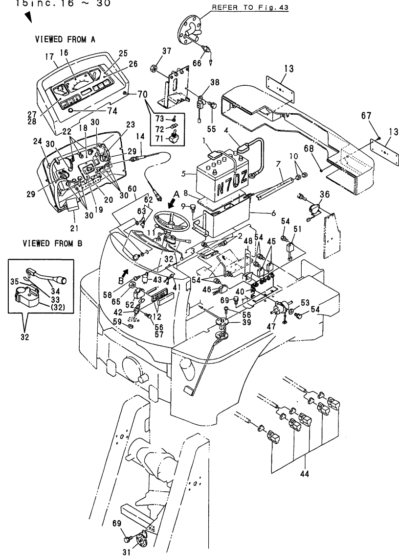
Fig.9 ELECTRIC PART
