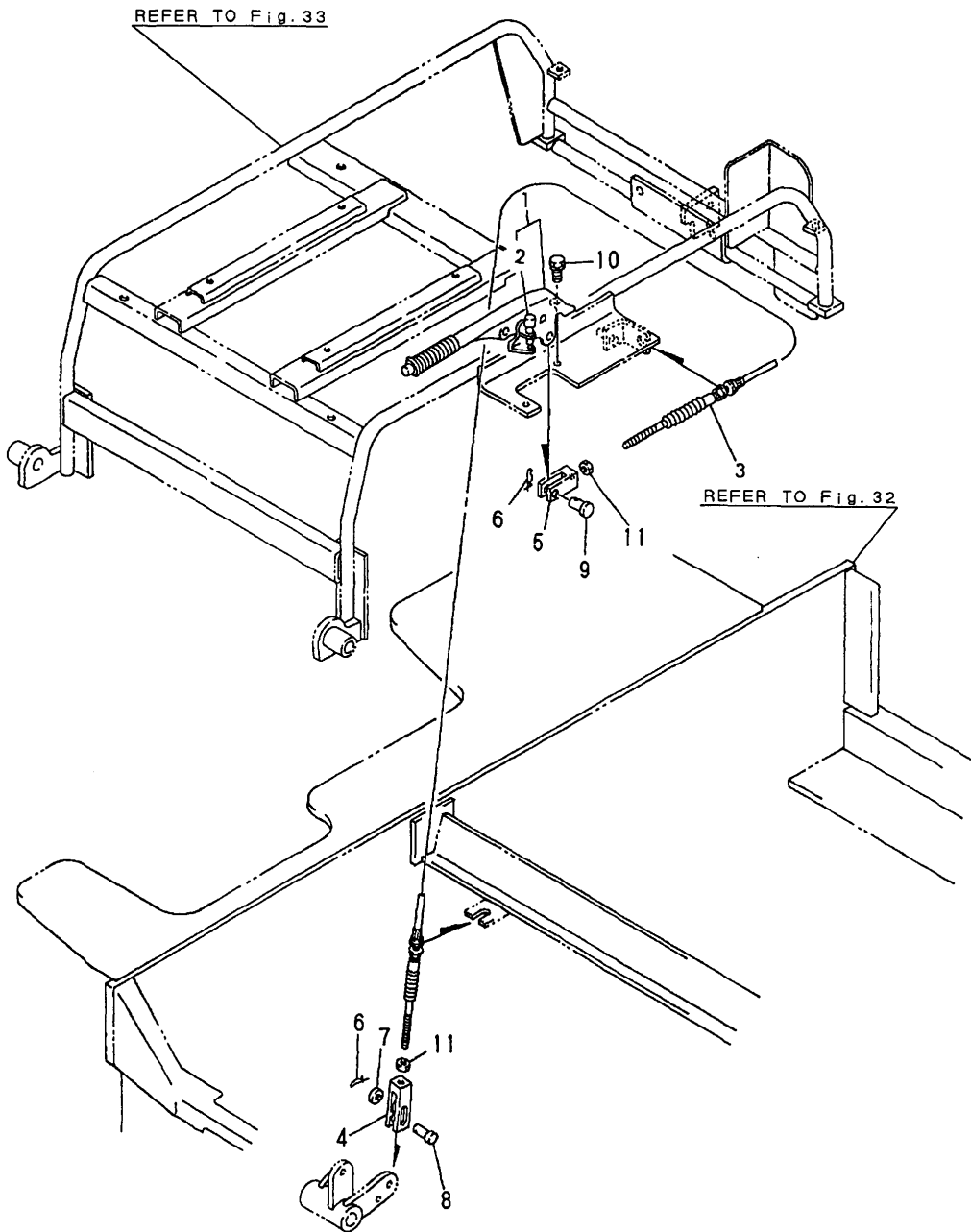
Fig.26 PARK BRAKE LEVER
