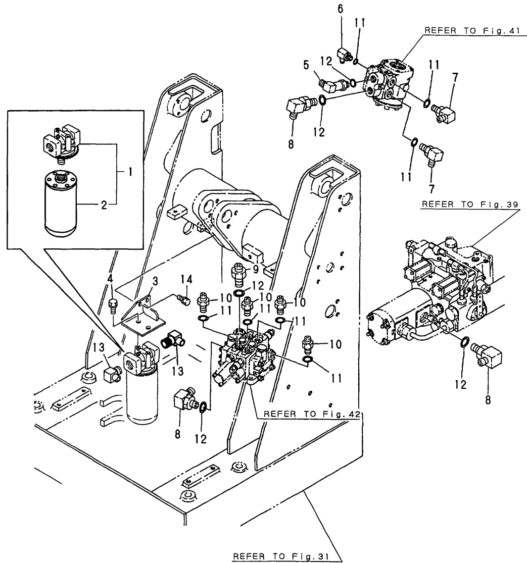
Fig.44 FILTER & PIPE FITTING
