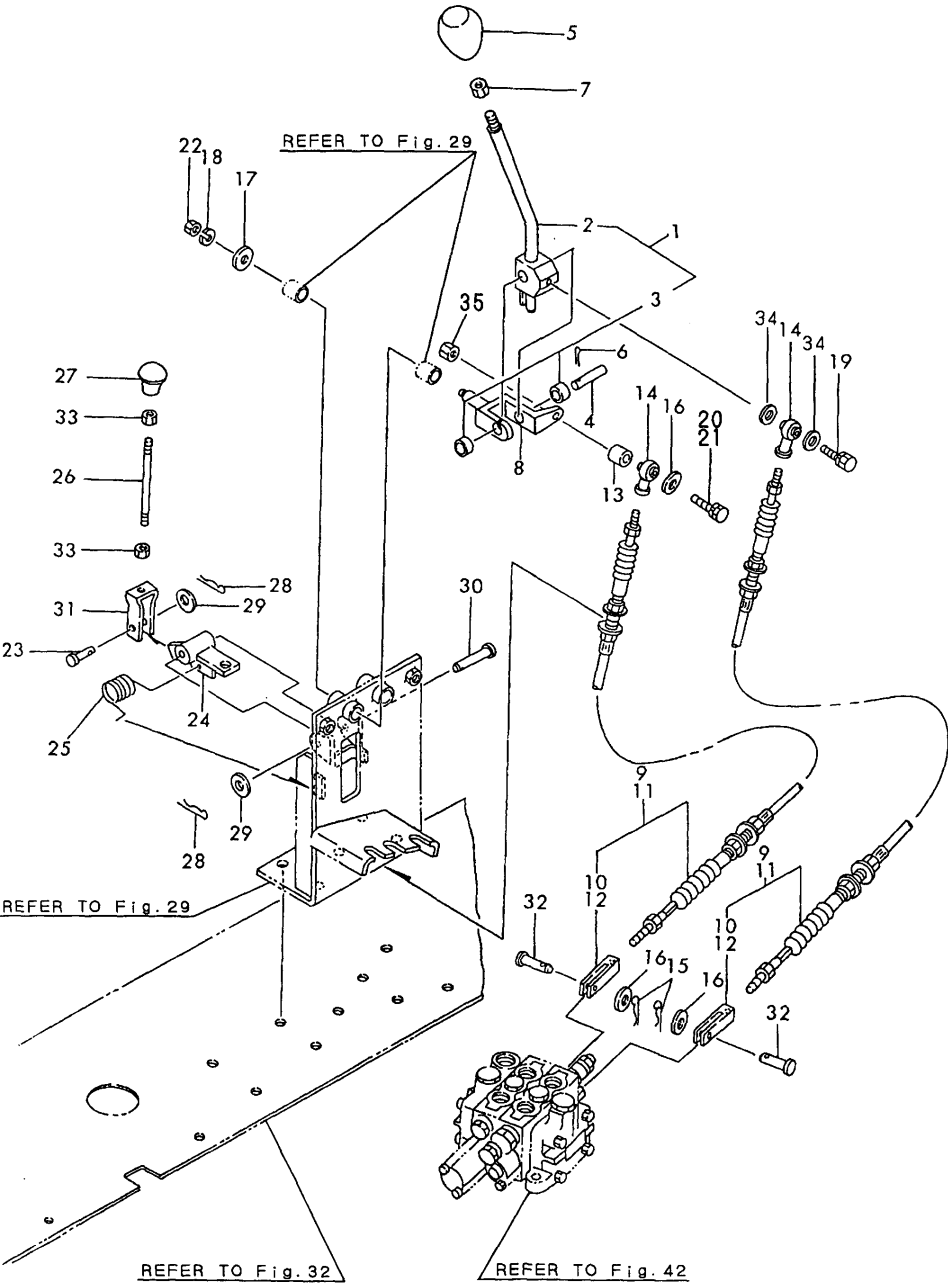
Fig.27 HYDRAULIC OIL CONTROL LEVER
