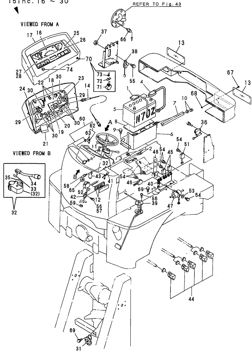
Fig.9 ELECTRIC PART
