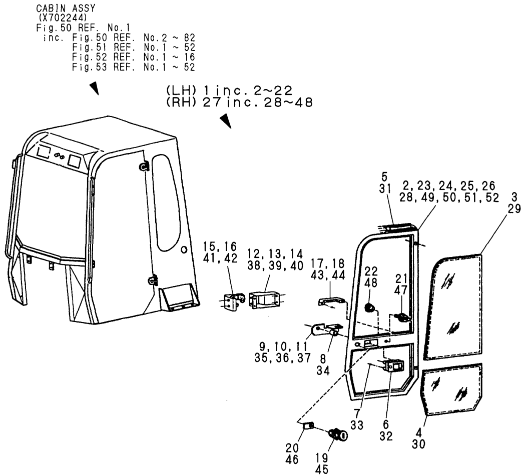
Fig.53 CABIN (4) (DOOR)
