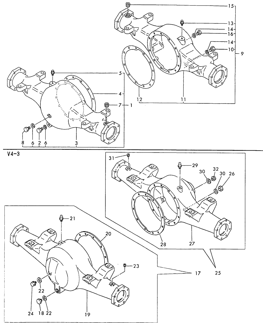
Fi g.20 AXLE CASE
