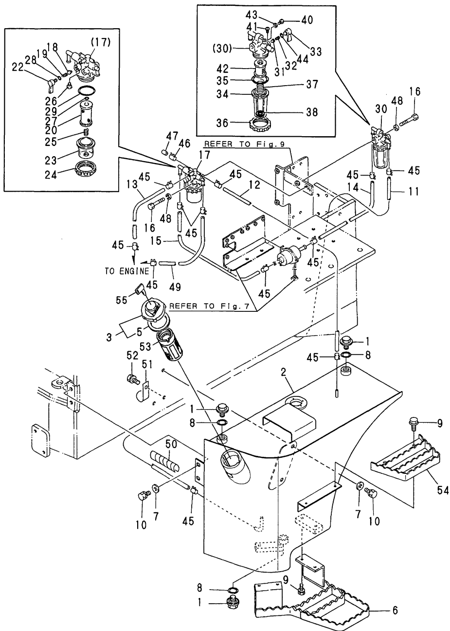
Fig. 8 FUEL TANK
