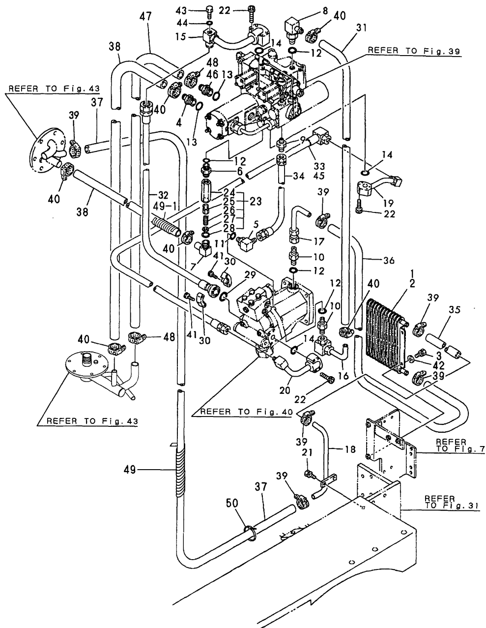
Fig. 45 HYD. OIL PIPING (HST)
