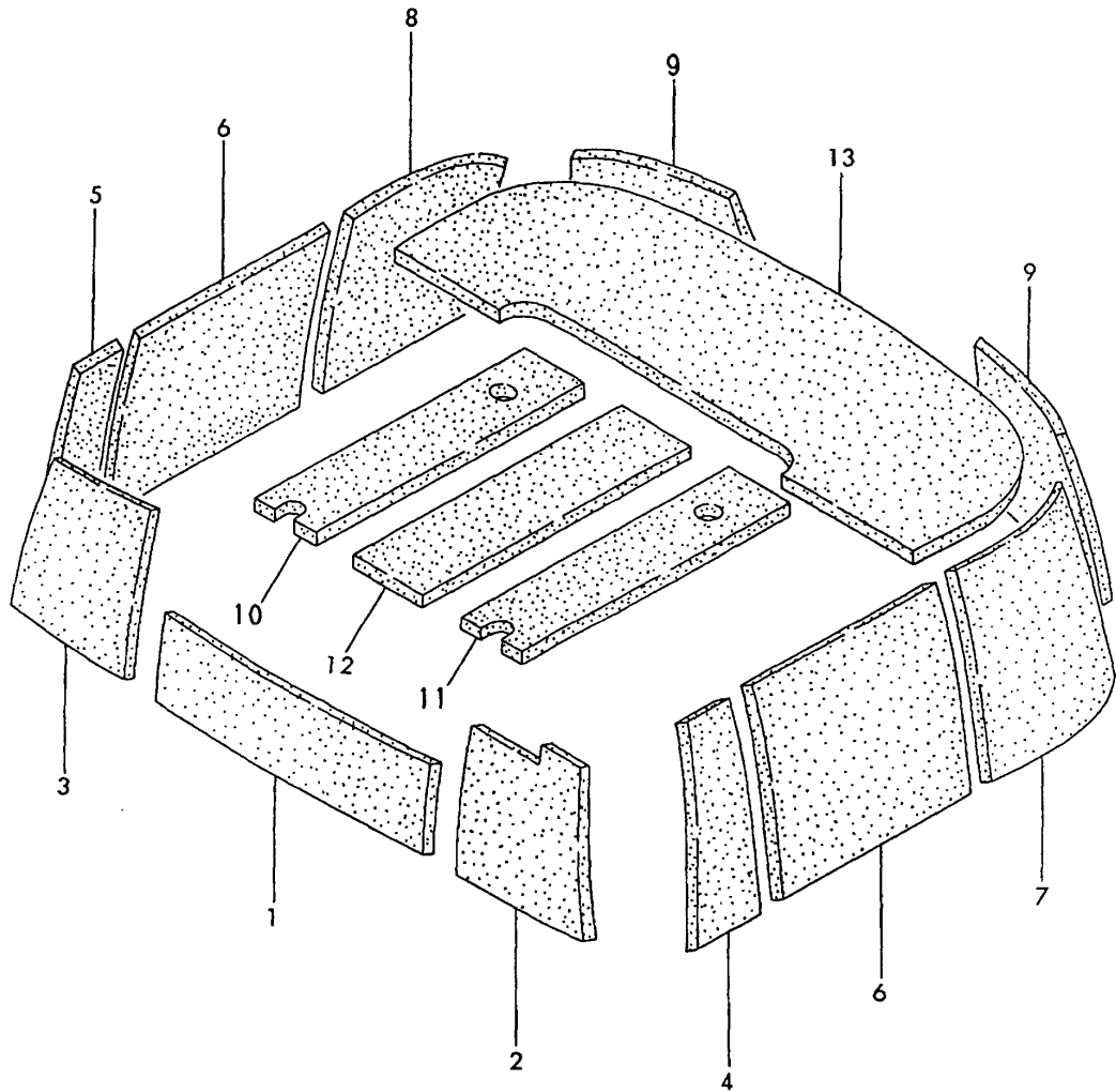
Fig.34 BONNET SOUNDPROOF MATERIAL
