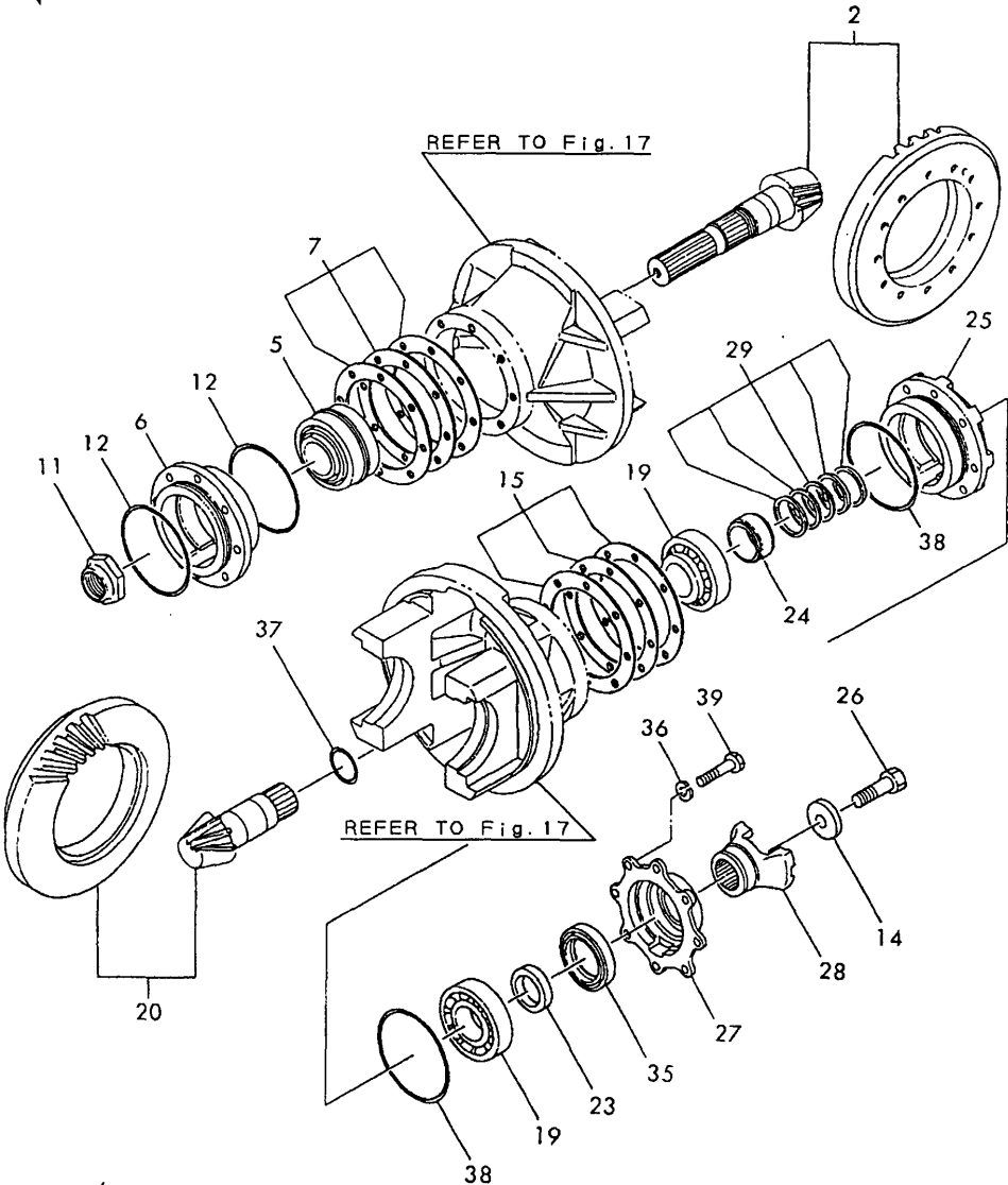
Fig.15 SPIRAL BEVEL GEAR (V4-3) 1 inc. 2 ~ 12
