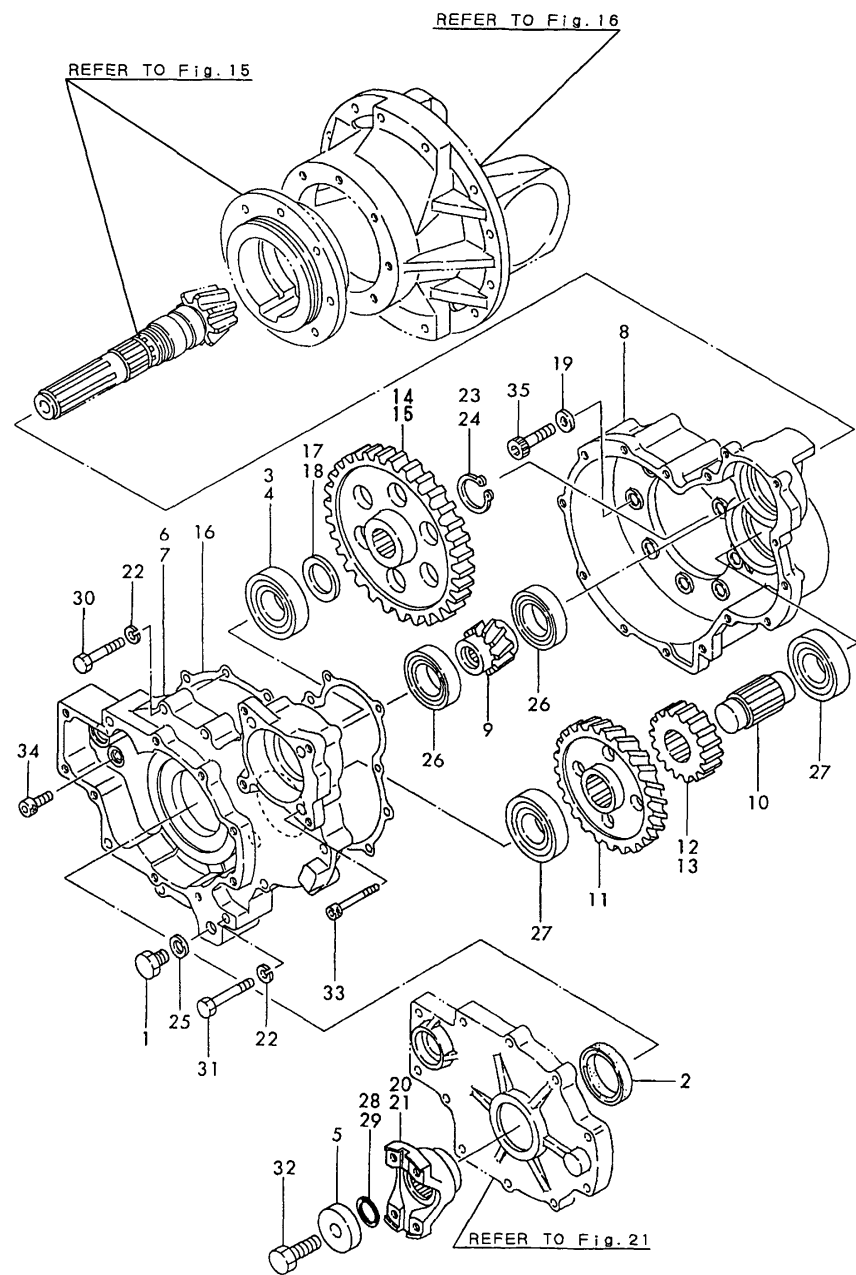
Fig.13 TRANSFER CASE
