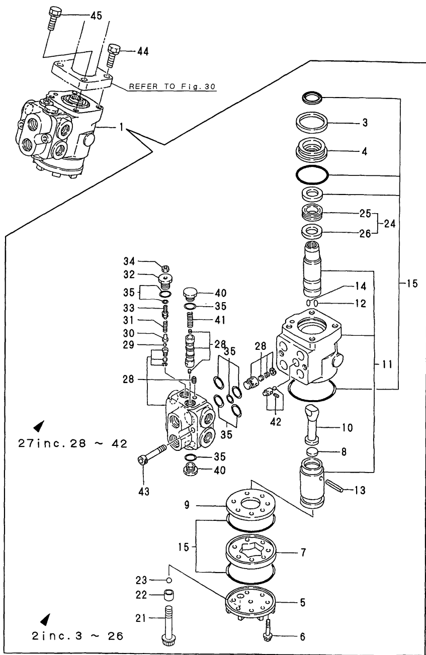
Fig.41 STEERING UNIT
