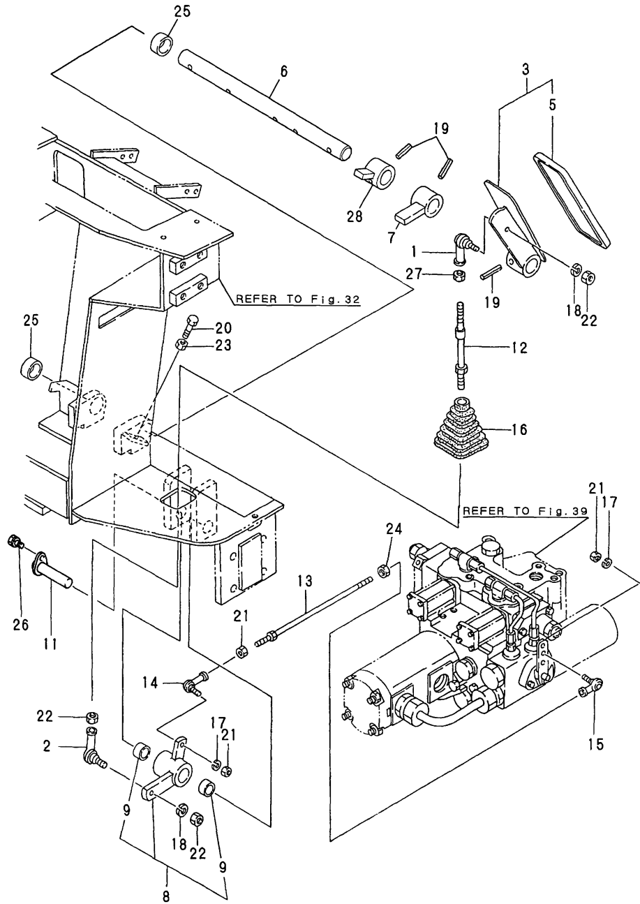
Fig.24 INCHING PEDAL
