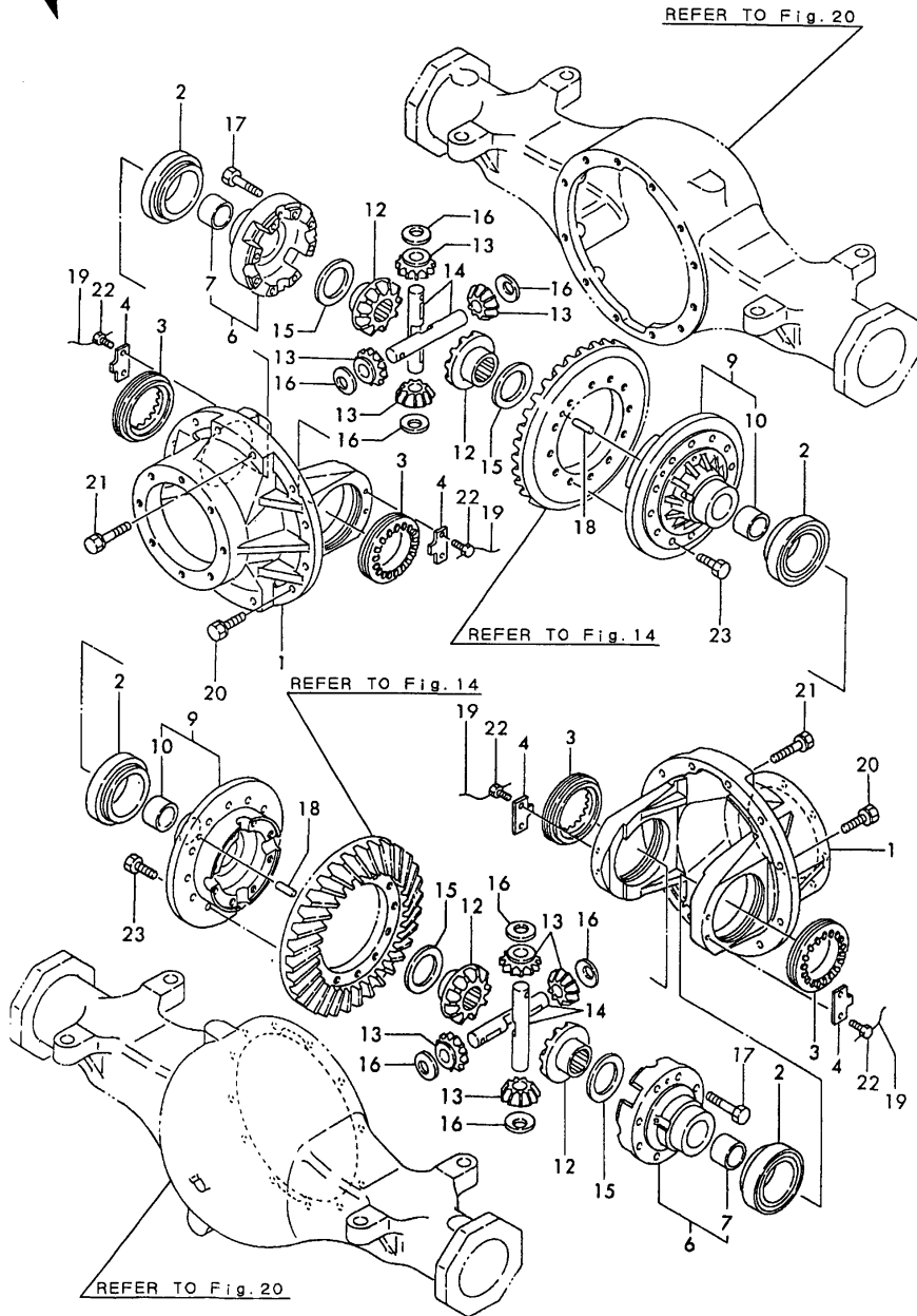
Fig. 16 DIFFERENTIAL GEAR (V3-3) 5inc. 6 ~ 17
