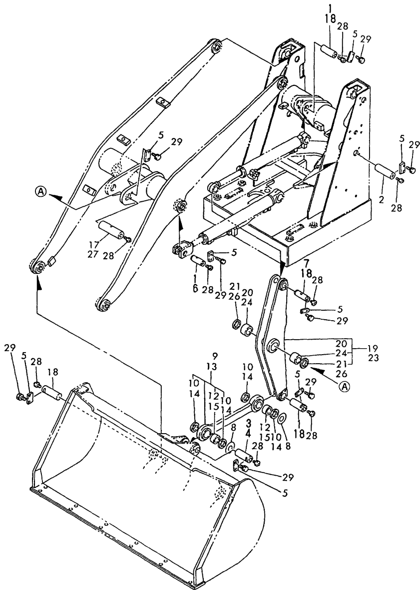
Fig.48 LOADER LINK
