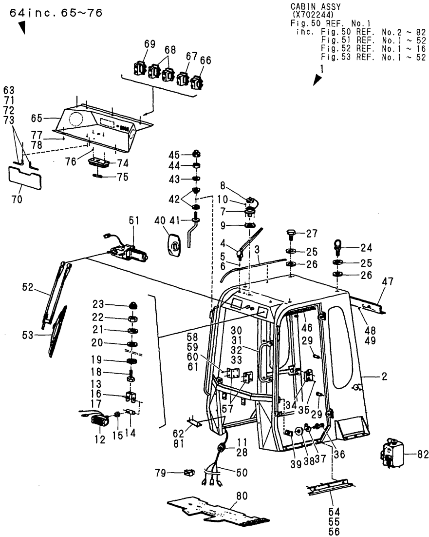
Fig.50 CABIN (1) (BODY)
