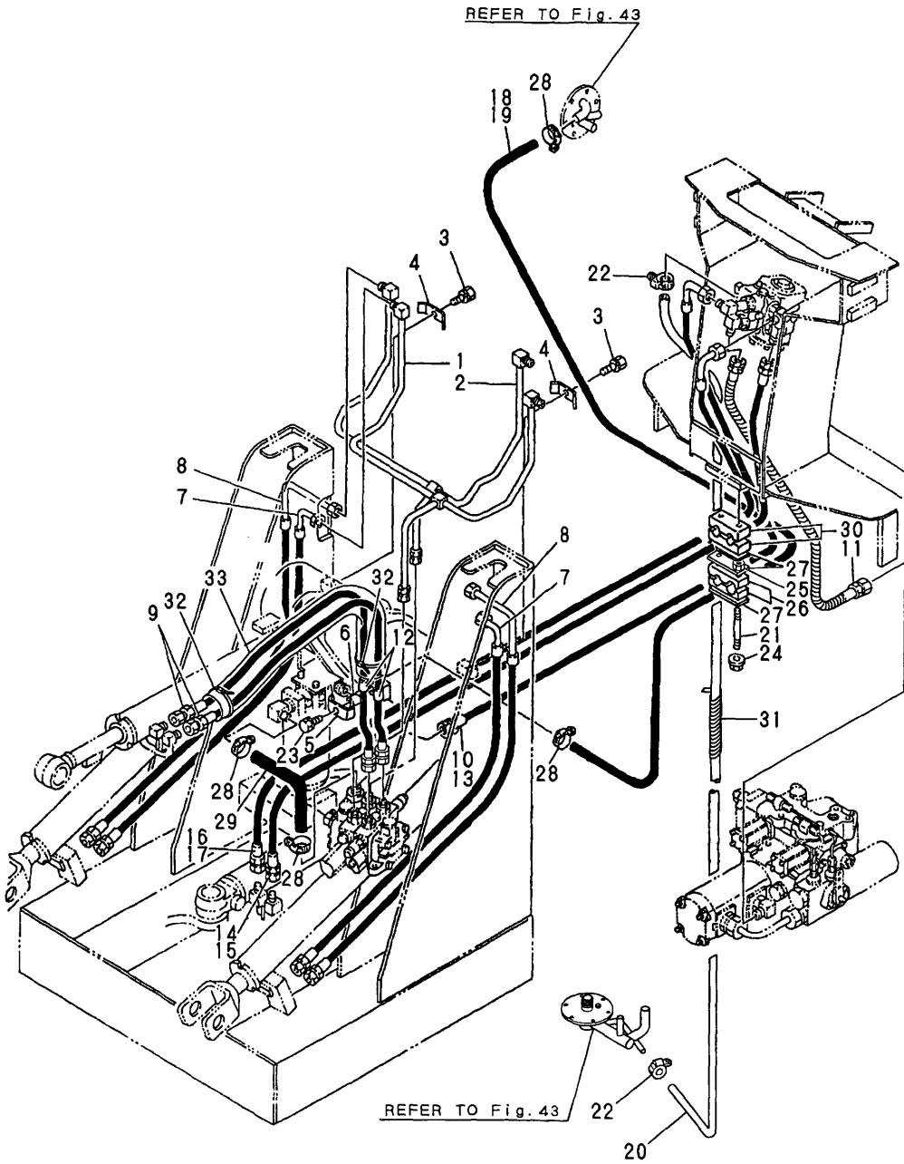
Fig.46 HYD.OIL PIPING (LOADER)
