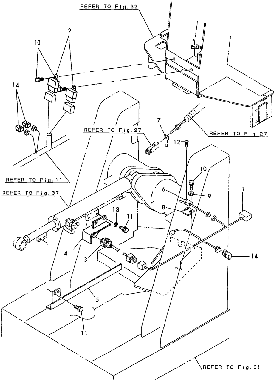
Fig.10 ELECTRIC PART (AUTO LEVELLER)
