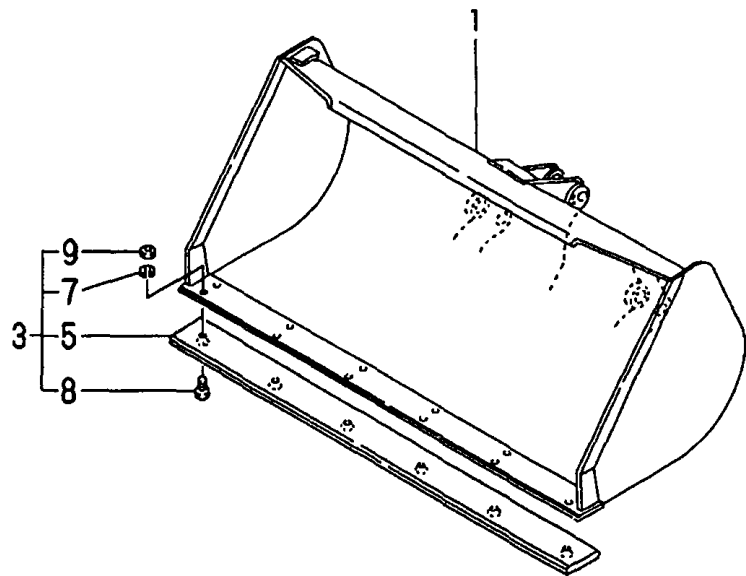
Fig.49 BUCKET
