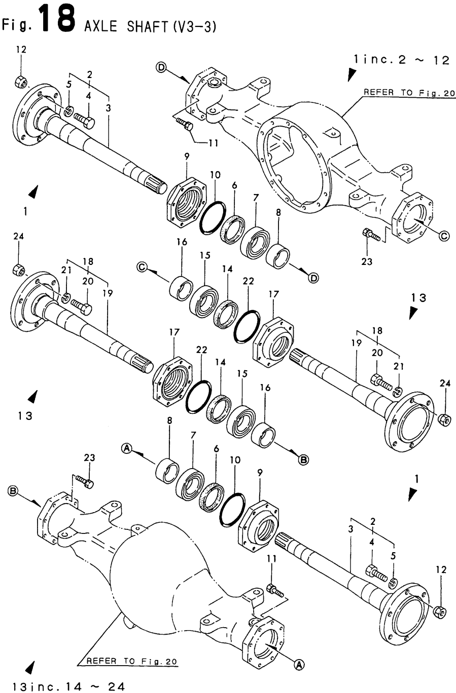
Fig.18. AXLE SHAFT(V3-3)
